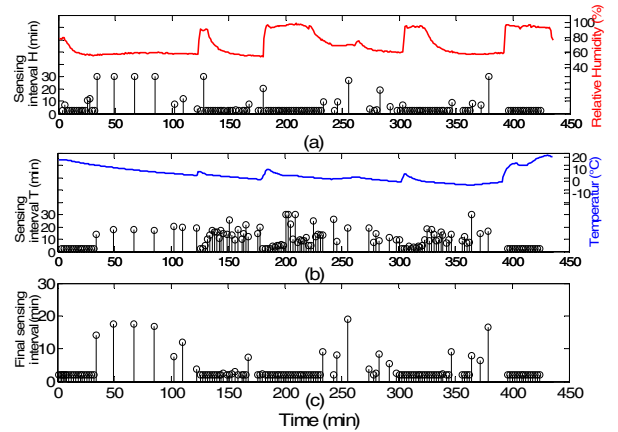
Fig. 6. Simulation results of adaptive data sensing intervals according to (a) relative humidity (b) temperature (c) final sensing interval. The sensing intervals in Fig 6(a) and (b) are calculated corresponding to the temperature and the relative
