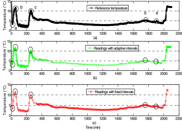
Fig. 9 Temperature sensor readings in zone A: (a) reference records with fixed interval of 2.5 min (b) records with adaptive sensing intervals (c) records with the same number of samples with (b), whereby the samples are evenly distributed in the entire process.
