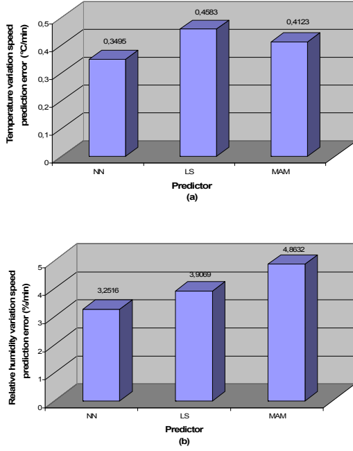
Fig. 4 Accuracy comparison of three predictors for (a) temperature and (b) relative humidity: neural networks (NN), least squares (LS) and modified Adams methods (MAM)
