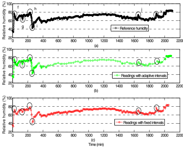
Fig. 10 Relative humidity sensor readings in zone A: (a) reference records with fixed interval of 2.5 min (b) records with adaptive sensing intervals (c) records with the same number of samples with (b), whereby the samples are evenly distributed in the entire process.
