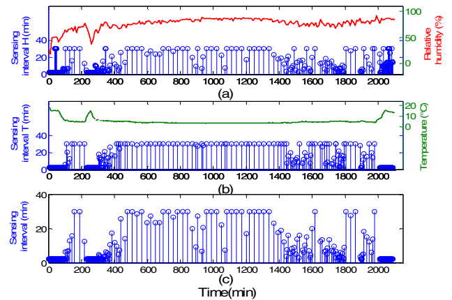
Fig. 8 Applied sensing intervals during the transport process (a) calculated necessary intervals for humidity (b) necessary intervals for temperature (c) final applied sensing intervals for both parameters
