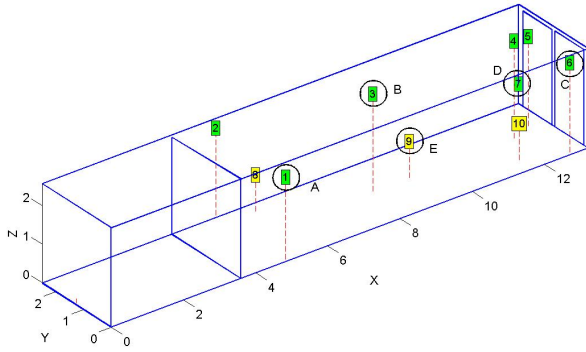
Fig.7. Scales of the container and the distribution of the sensor nodes in the fresh area (A-E are the five zones for algorithm test)
