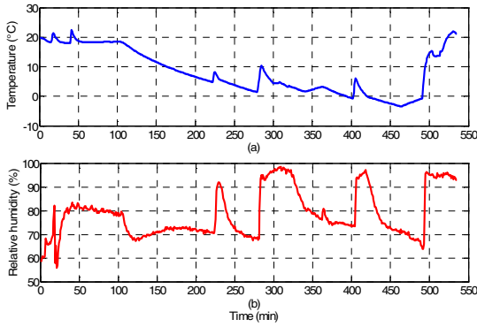
Fig. 3 Input data of the simulation test (a) Temperature (b) Relative humidity
