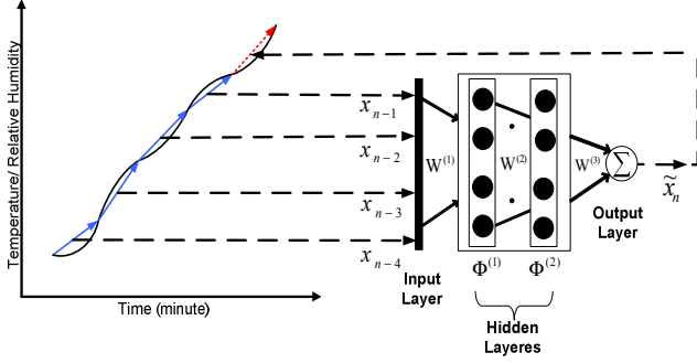
Fig. 2 Applied neural network architecture to predict the variation of the environmental parameters
