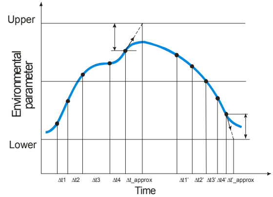
Fig. 1 Principle of the adaptive sensing interval algorithm
